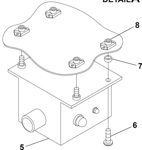
FLIGHT DATA RECORDER Figure 01. (Sheet 1)
