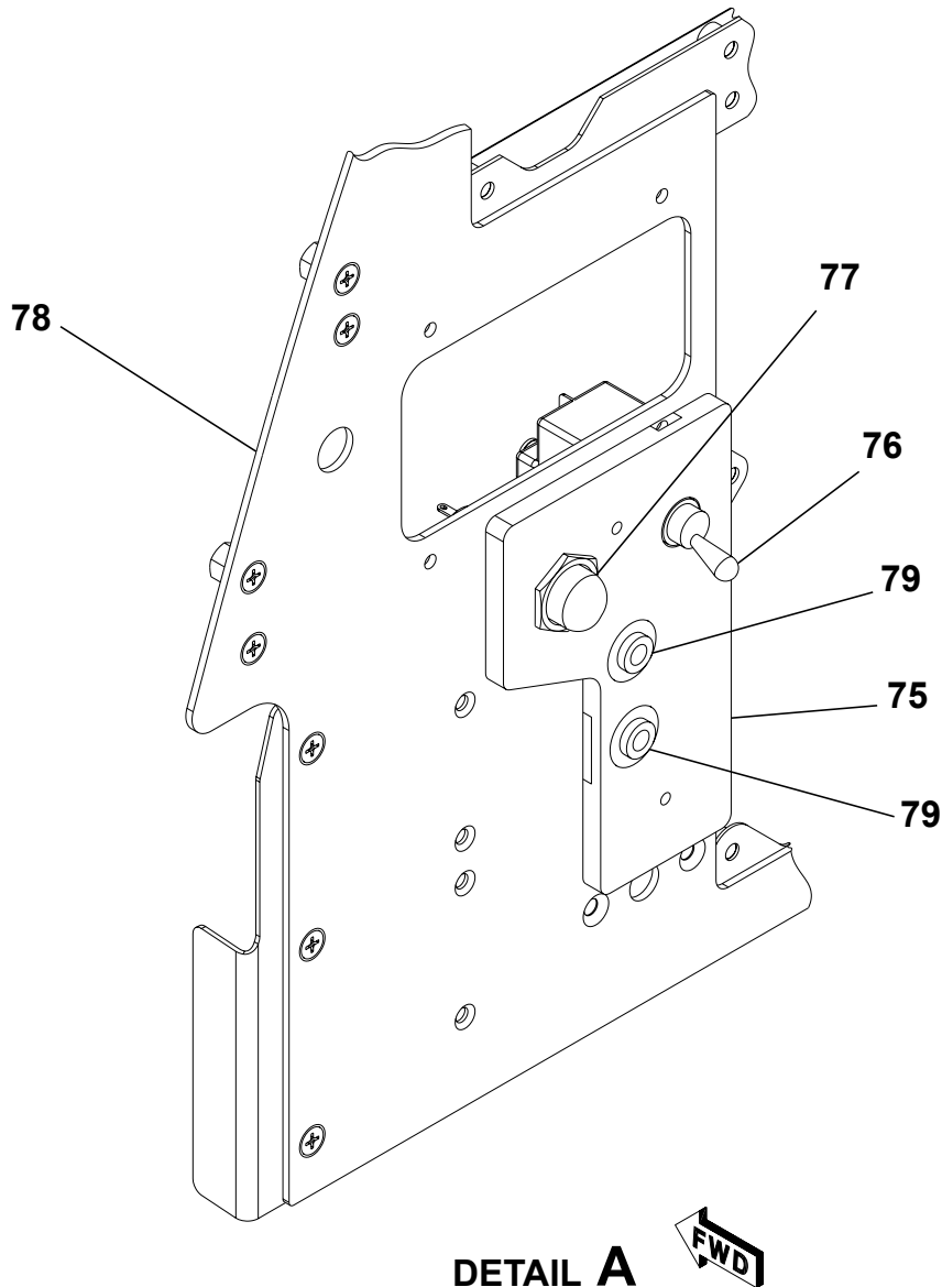
SWITCH PANEL ASSEMBLY Figure 01A. (Sheet 2)
