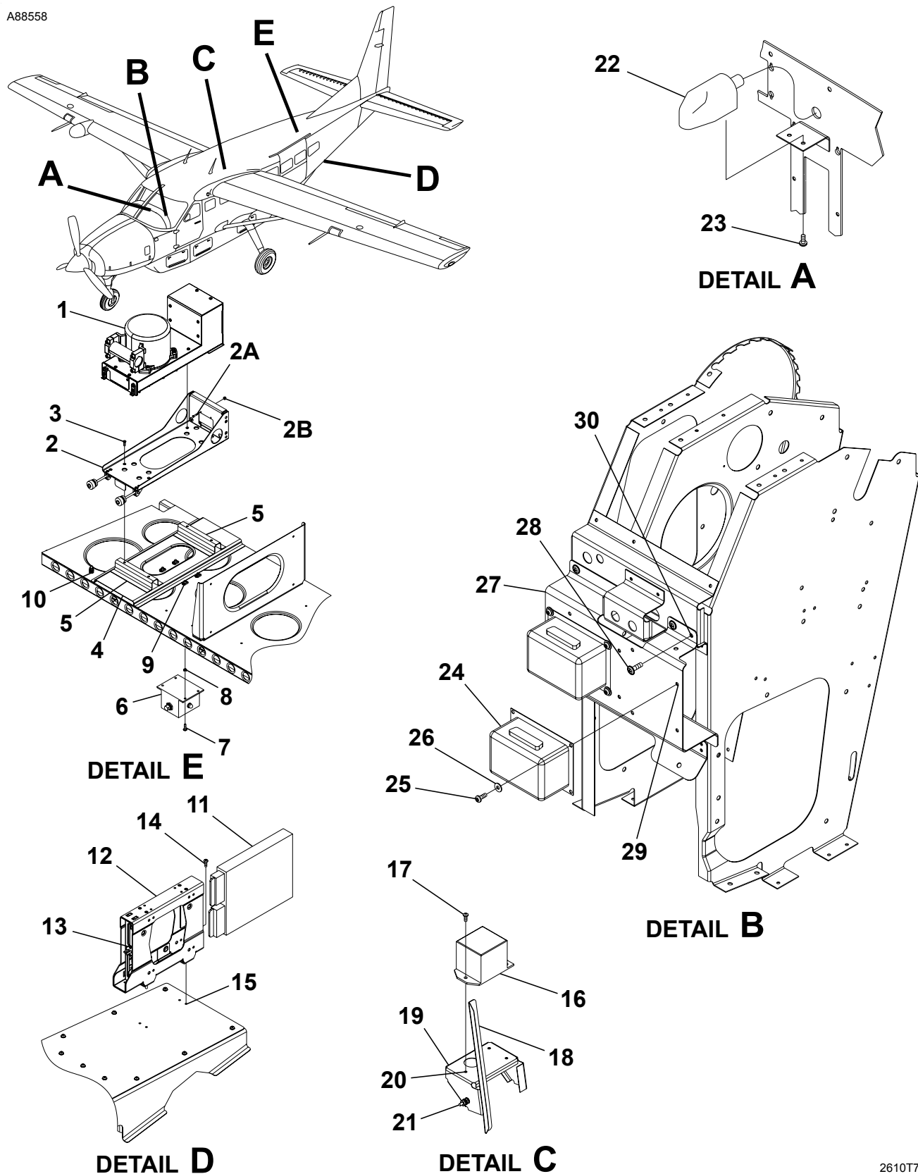
COCKPIT VOICE DATA RECORDER INSTALLATION Figure 02. (Sheet 1)
