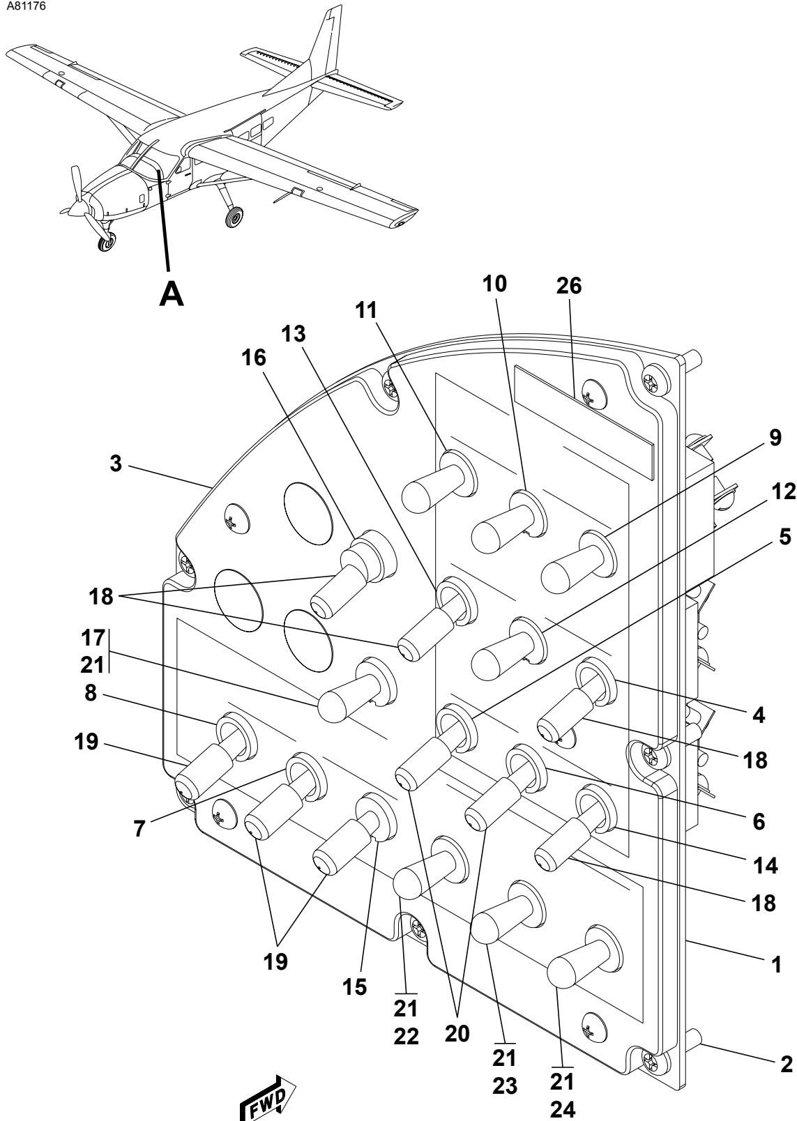
SWITCH PANEL ASSEMBLY Figure 01A. (Sheet 1)
